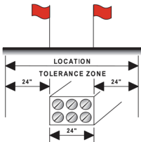
Large pipe or multiple utilities of known size
